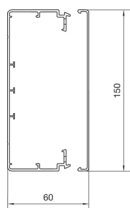
LF6015009001
